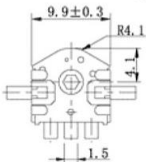
Shaft hole shape and dimension
